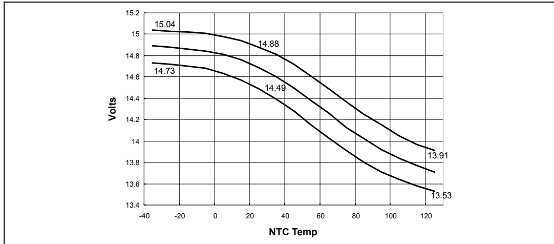
Figure 5. Set-point voltages vs. mounting tab temperature (TS-Open)
