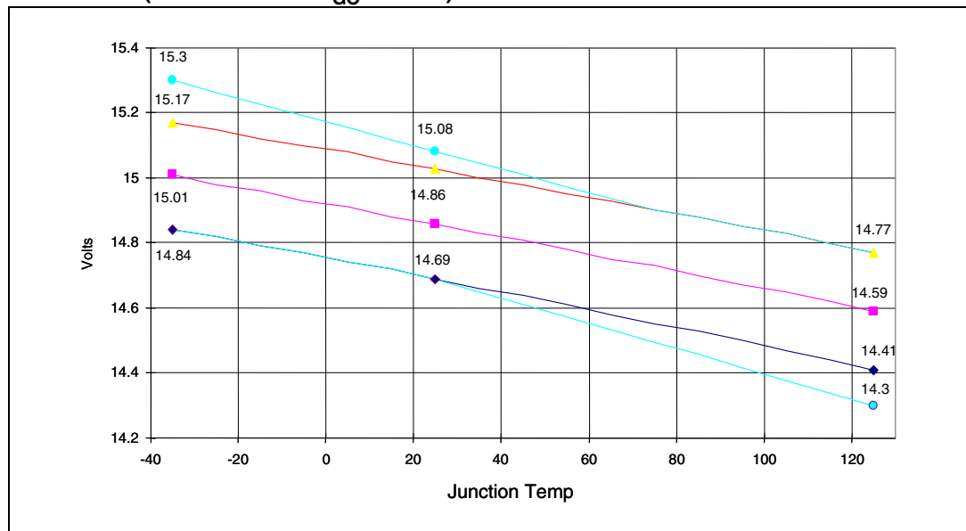
Figure 3. Set-point voltage vs. mounting tab temperature (10k \Omega between V_{GO} and TS)
