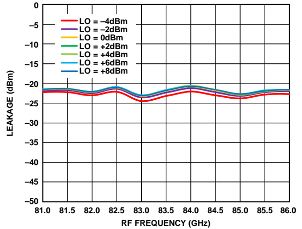
Figure 78. 6 \times LO Leakage at RFOUT vs. RF Frequency at Various LO Powers, I_{FIN} = 5 \text{ dBm} , IF = 2000 \text{ MHz} , LSB
