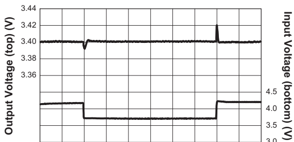
V BAT Line Transient Response LDO1 (V BAT = 3.7V to 4.2V; I OUT1 = 150mA; V OUT1 = 3.4V)
