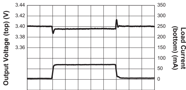
Load Transient Response LDO1 (10mA to 75mA; V BAT = 3.6V; V OUT = 3.4V)
