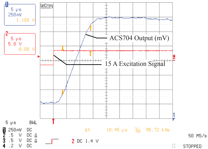
Step Response of ACS704ELC-015 at T_A=25^\circ\text{C}
