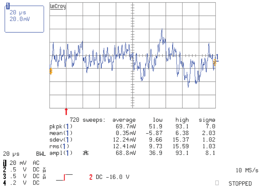
Typical Peak-to-Peak Noise of ACS704ELC-015 at T_A=25^\circ\text{C}
