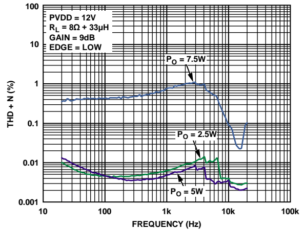
Figure 12. THD + N vs. Frequency; R_L = 8\Omega ; PVDD = 12 V; P_O = 2.5\text{ W} , P_O = 5\text{ W} , P_O = 7.5\text{ W}
