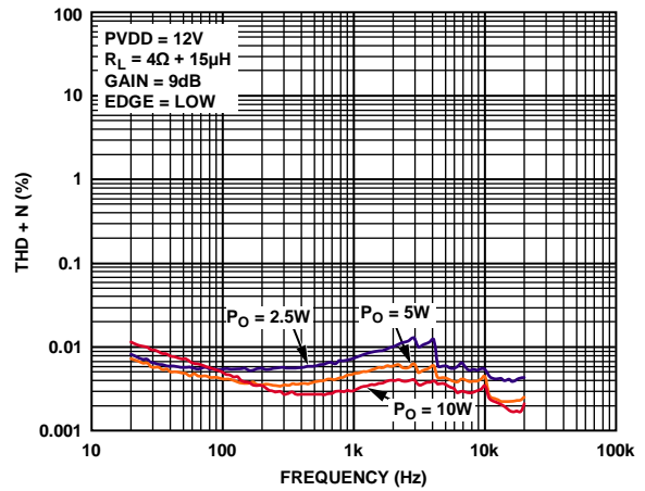
Figure 13. THD + N vs. Frequency; R_L = 4\Omega ; PVDD = 12 V; P_O = 2.5\text{ W} , P_O = 5\text{ W} , P_O = 10\text{ W}
