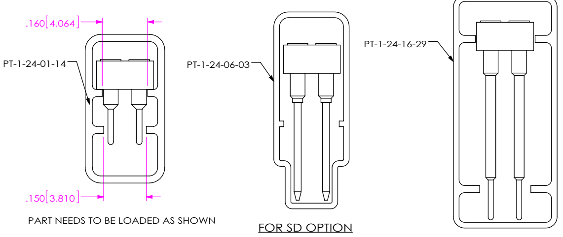
PACKAGING VIEWS (SEE NOTE 10 & TABLE 3)
