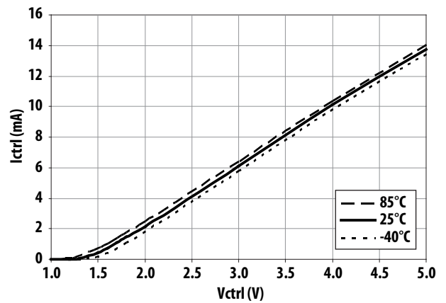
Figure 28. Current ( I_{ctrl} ) vs Control Voltage and Temperature
