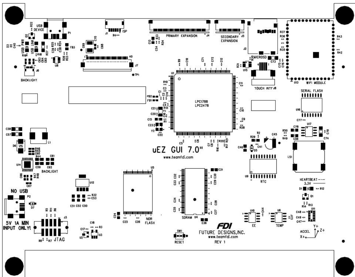
Figure 2 – uEZGUI-2478-43WQS Component View
